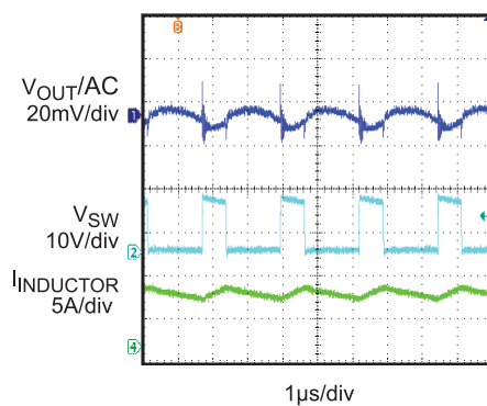
Output Ripple Voltage Full Load
