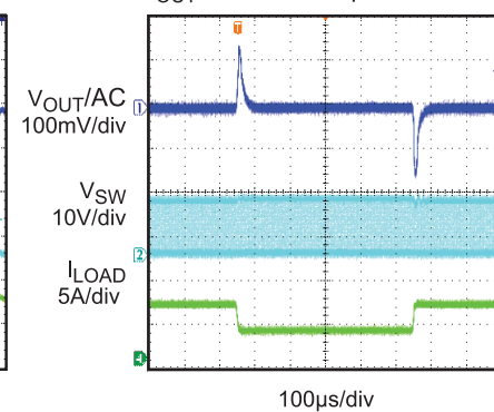
Load Transient Response I_{OUT}=3A to 6A 1A/\mu s
